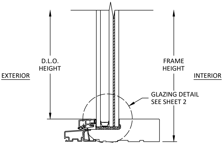
B 6 VERTICAL SECTION SILL INSULATED GLASS SHOWN
