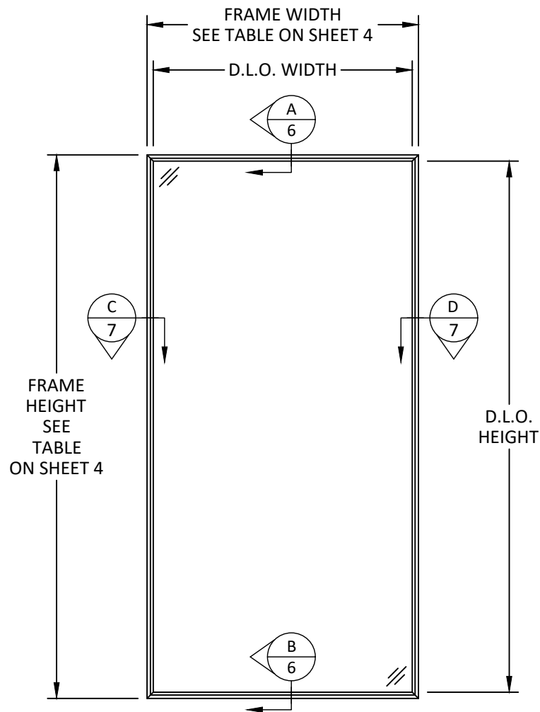
TYPICAL ELEVATION
