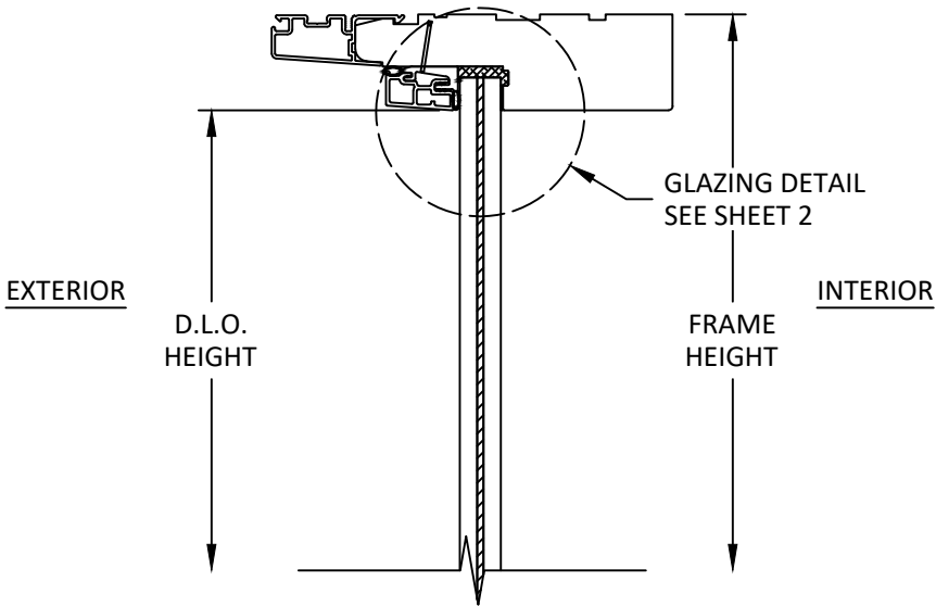
A 6 VERTICAL SECTION HEAD MONO. GLASS SHOWN
