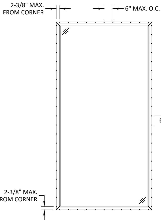
ANCHOR LAYOUT NAILING FLANGE
